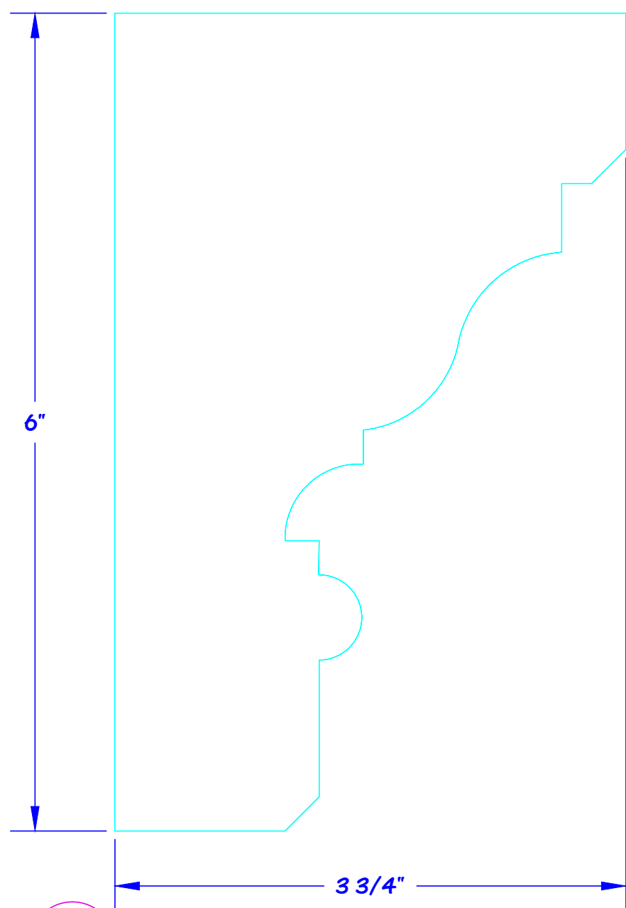
4 LOWER CROWN MLD FULL SCALE
