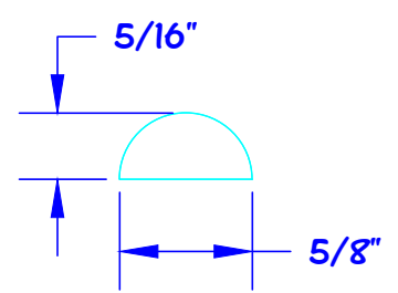
2 HALF ROUND MLD FULL SCALE
