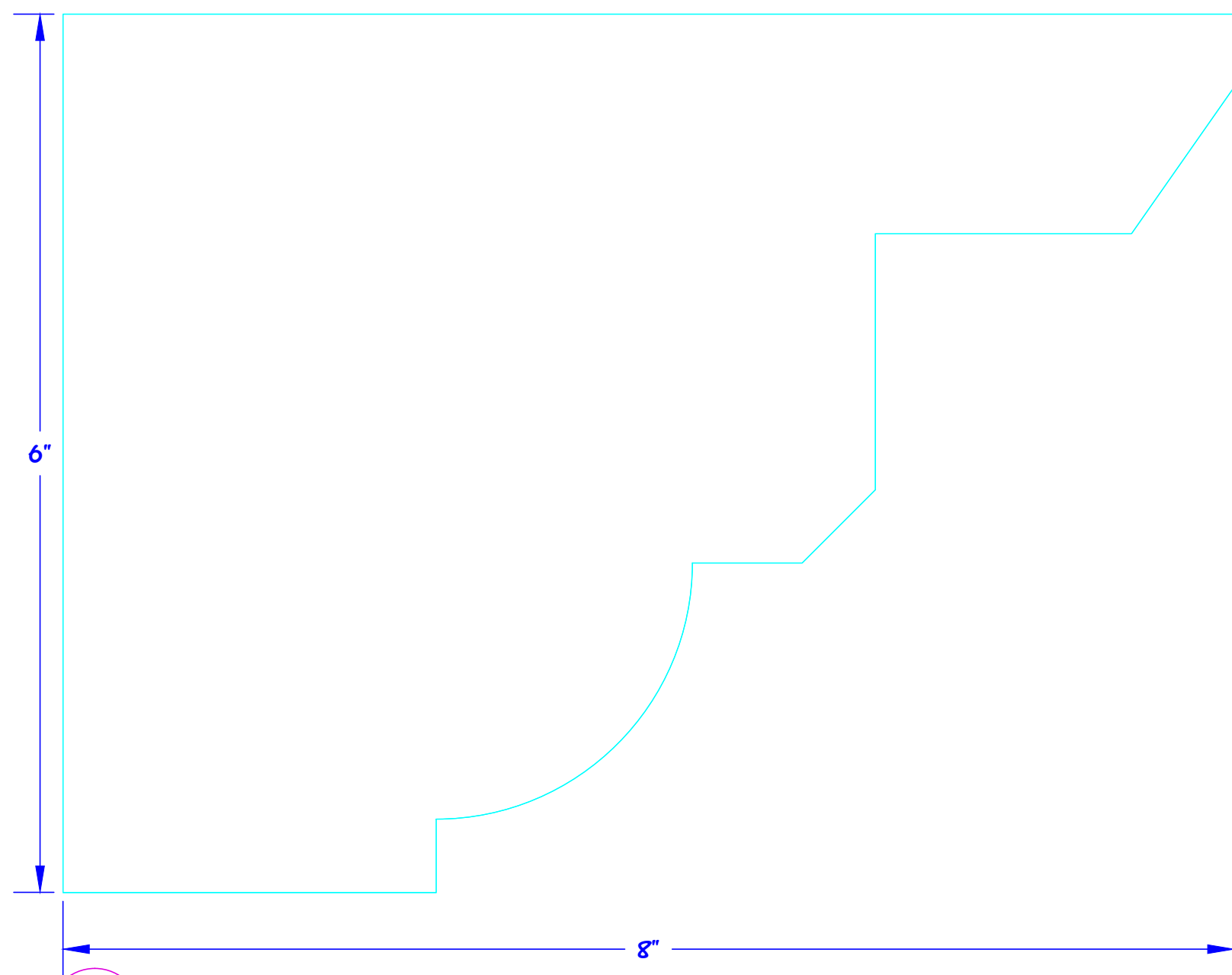
3 UPPER CROWN MLD FULL SCALE
